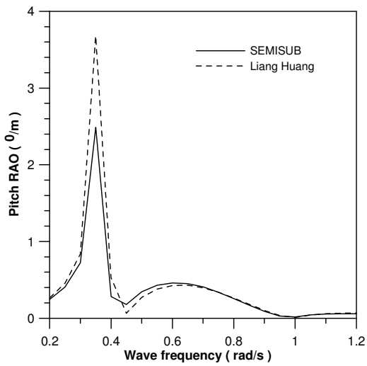
(c) Pitch RAO
