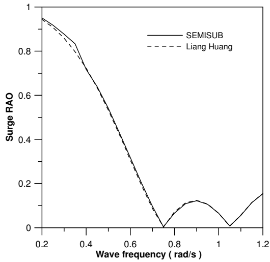
(a) Surge RAO
