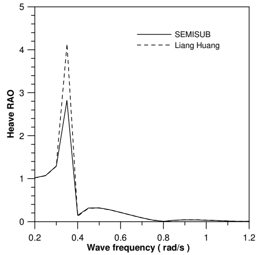
(b) Heave RAO
